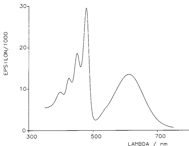
Figure 6. UV/Vis absorption spectrum of 13a (color coordinates x = 0.3091 , y = 0.4071 , Y = 53.01 , 2^\circ , normlight C at T_{\min} = 0.1 ) in chloroform
