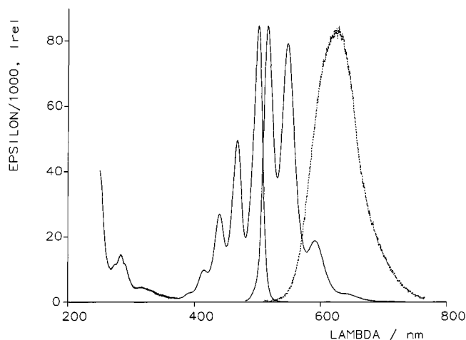
Figure 5. UV/Vis absorption and fluorescence spectra of 11a (color coordinates x = 0.3711 , y = 0.3808 , Y = 90.66 , 2^\circ , normlight C at T_{\min} = 0.1 ) in chloroform; (···): solid-state fluorescence
