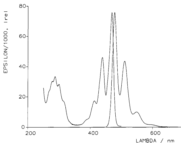
Figure 4. UV/Vis absorption and fluorescence spectra of 5a (color coordinates x = 0.3658 , y = 0.4150 , Y = 97.29 , 2^\circ , normlight C at T_{\min} = 0.1 ) in chloroform
