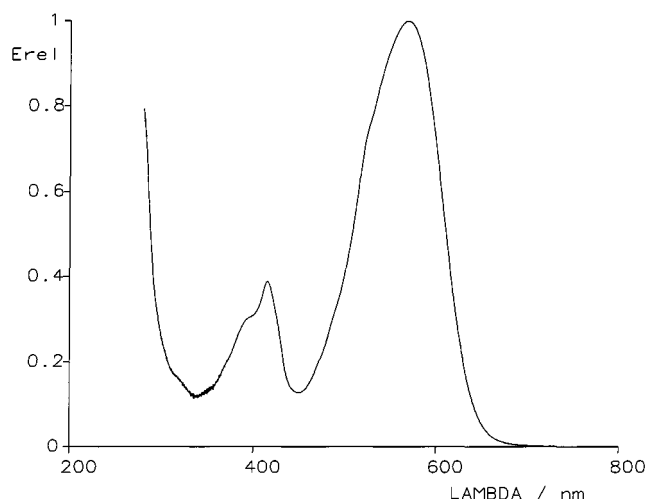
Figure 9. UV/Vis absorption spectrum of a mixture of 17c and 18c (color coordinates x = 0.2761 , y = 0.1731 , Y = 23.54 , 2^\circ , normal light C at T_{\min} = 0.1 ) in chloroform
