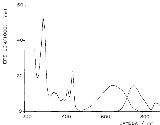
Figure 3. UV/Vis absorption and fluorescence spectra of 14a (color coordinates x = 0.2489 , y = 0.3507 , Y = 59.04 , 2^\circ , normlight C at T_{\min} = 0.1 ) in chloroform
