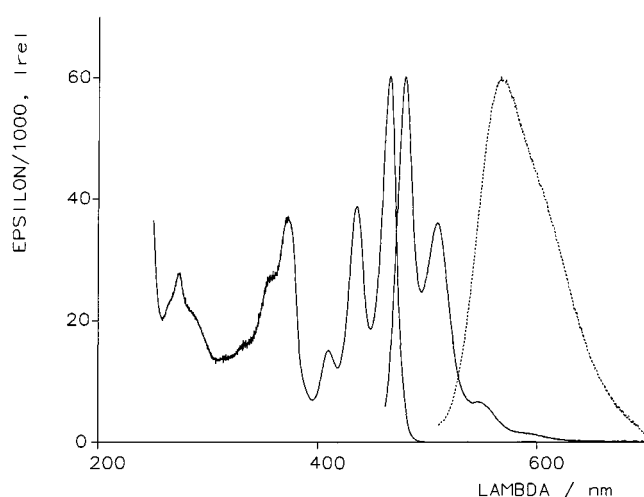
Figure 2. UV/Vis absorption and fluorescence spectra of 3a (color coordinates x = 0.3637 , y = 0.4156 , Y = 97.40 , 2^\circ , normlight C at T_{\min} = 0.1 ) in chloroform; (···): solid-state fluorescence
