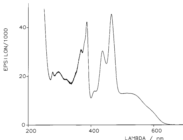
Figure 7. UV/Vis absorption and fluorescence spectra of 15a (color coordinates x = 0.4091 , y = 0.3951 , Y = 64.71 , 2^\circ , normlight C at T_{\min} = 0.1 ) in chloroform
