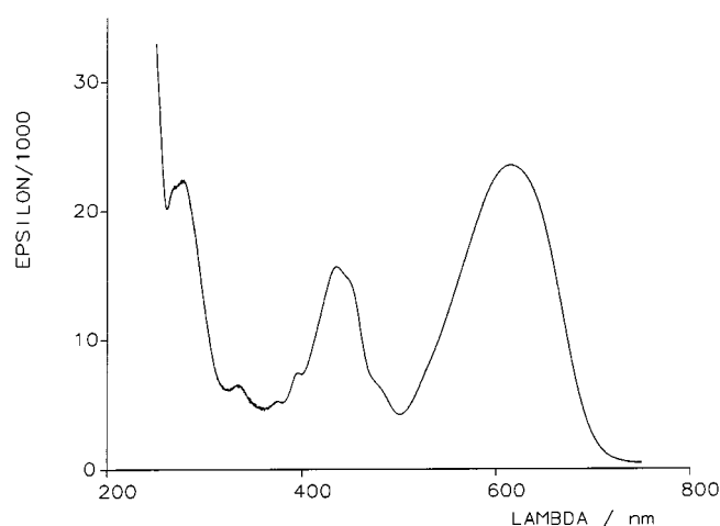
Figure 8. UV/Vis absorption spectrum of 10a (color coordinates x = 0.2142 , y = 0.3240 , Y = 29.78 , 2^\circ , normlight C at T_{\min} = 0.1 ) in chloroform
