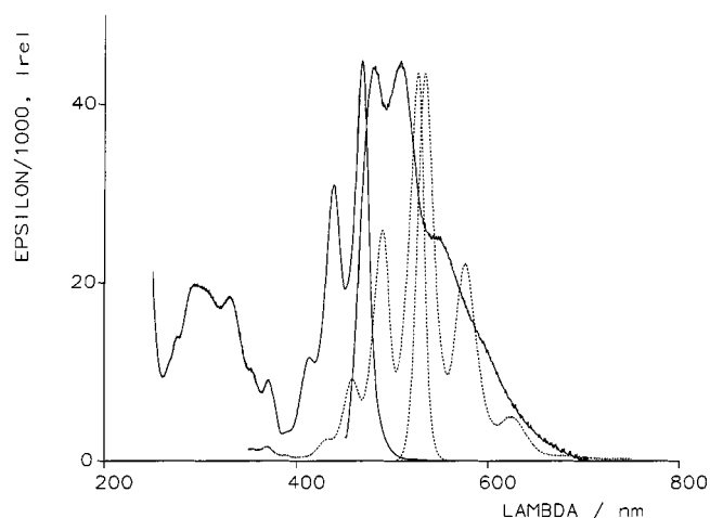
Figure 1. UV/Vis absorption and fluorescence spectra of 2a (color coordinates x = 0.3767 , y = 0.4315 , Y = 96.49 , 2^\circ , normlight C at T_{\min} = 0.1 ) in chloroform compared to 1a [ R^1 = \text{CH}(\text{C}_6\text{H}_{13})_2 , half of the molar absorptivity of 1a ] (···)
